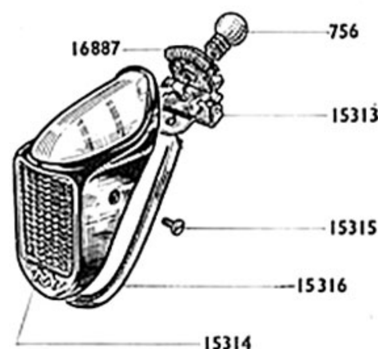
Phare complet LUXOR 17033
